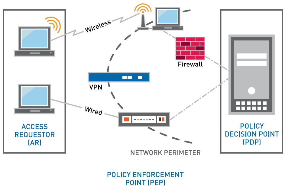
Figure 1: TNC Architecture—from TNC: Open Standards for Network Access Control
